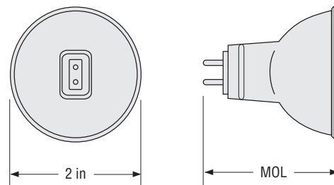
GU5.3 Base
