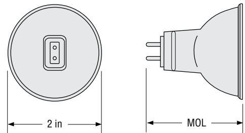
GU5.3 Base
